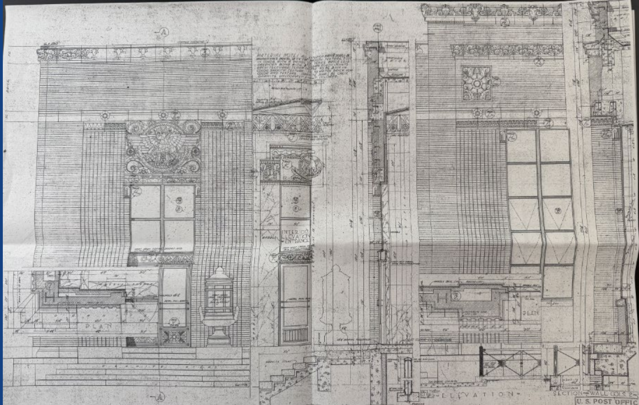
ELEVATION OF ENTRANCE - SECTION THRU ENTRANCE - THREE QUARTER INCH SCALE DETAILS OF EXTERIOR, COLS 1 AND 2
